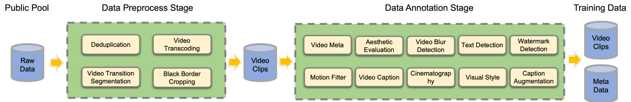
Figure 2: Overview of data curation pipeline. The data preprocessing stage extracts well-segmented video clips from raw source videos in the data pool. In the data annotation stage, each video clip is annotated with a variety of attributes, forming a comprehensive metadata database. This metadata database enables the convenient and flexible assembly of training datasets to support various training stages and objectives.
