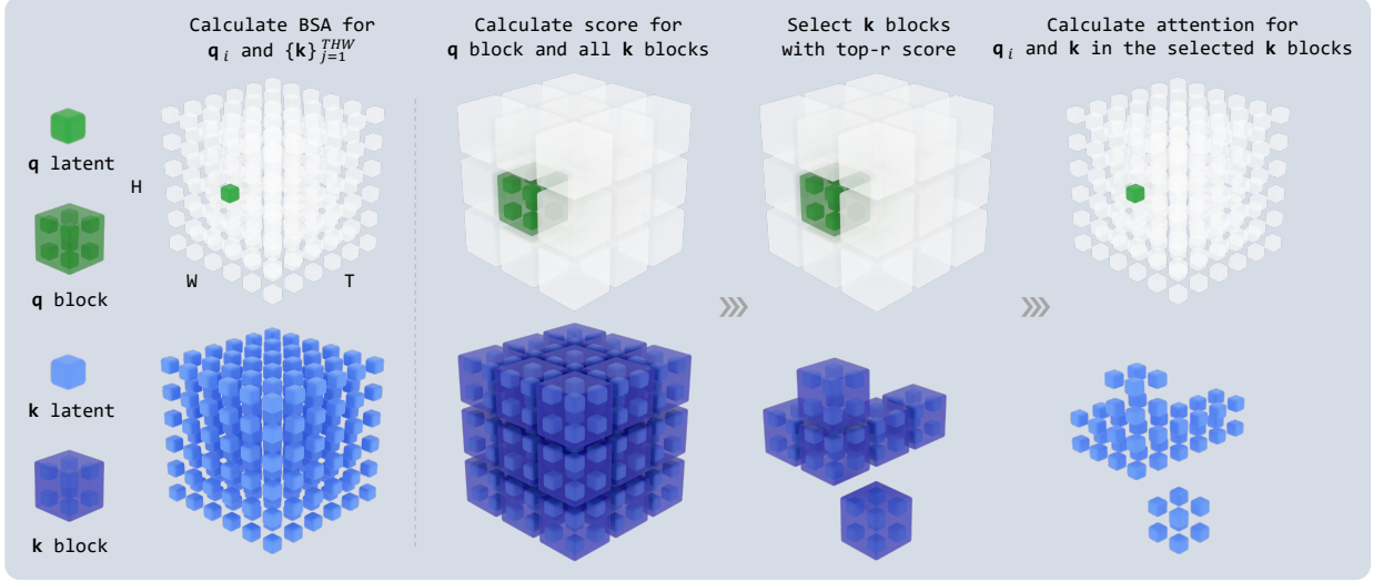
Figure 12: Illustration of 3D block sparse attention for query q_i and keys \{k_j\}_{j=1}^{THW} . (a) Partition q_i and all k_j into non-overlapping 3D blocks of size t \times h \times w . The block containing q_i is identified, and a similarity score is computed between this query block and each key block using their average values. (b) Select the top- r key blocks with the highest similarity scores. (c) Compute the standard attention between q_i and all keys within the selected r key blocks.
