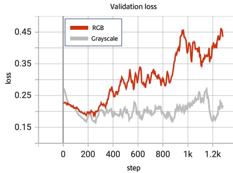
Figure 20: MQ Reward model validation loss curve
