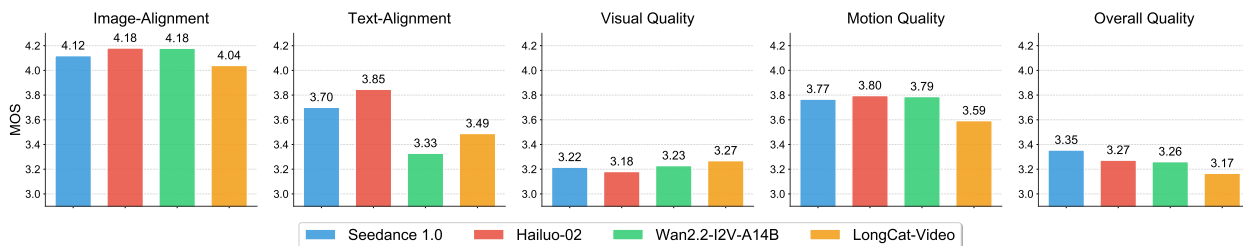
Figure 16: Image-to-Video MOS evaluation results on our internal benchmark.
